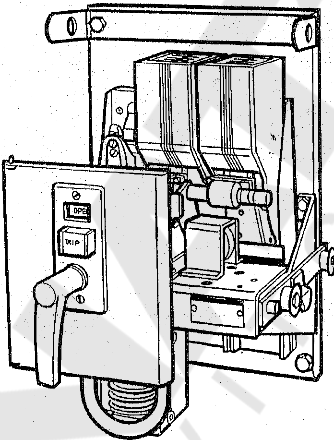
DB-25 Front View
