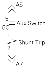
Figure 6. Shunt Trip connections to the secondary disconnect.
