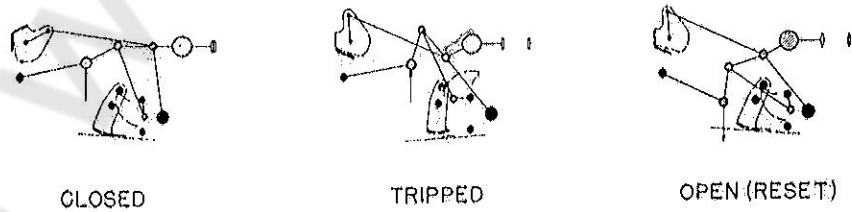
Cross-Sectional View of Type DB-50 Circuit Breaker
