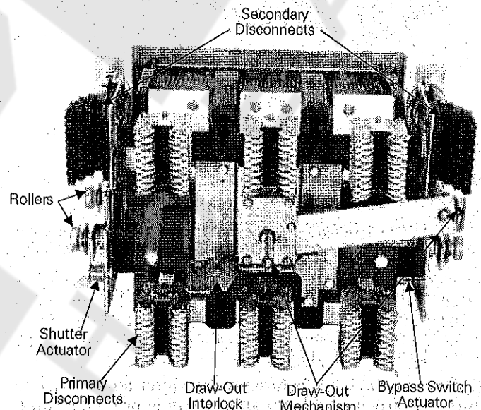
Figure 1. Rear view of the Power Break® II draw-out device.
