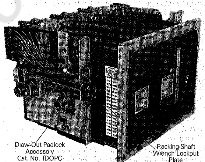
Figure 2. Left side of the device, showing the padlock accessory and racking shaft lockout plate.
