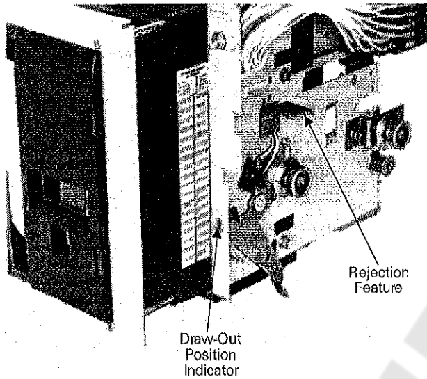
Figure 3. Right side of the device, showing the rejection feature, draw-out position indicator, and electric operator cutoff switch.
