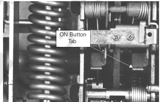
Figure 2. Tab on the breaker mechanism engaged by the On button.
