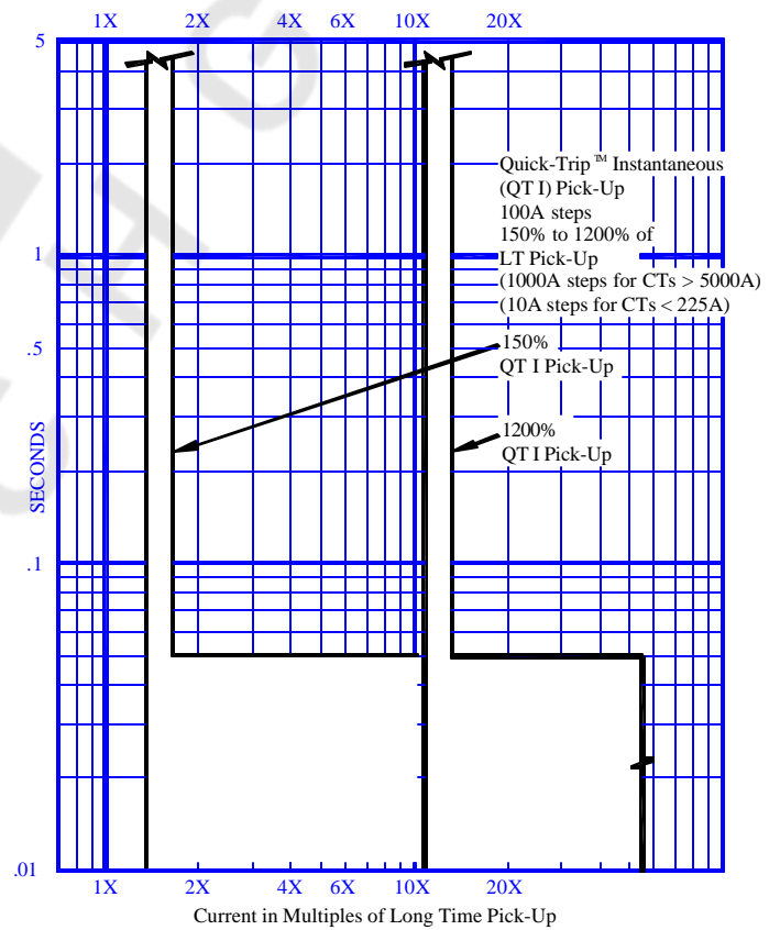
Quick-Trip™ Instantaneous Time Current Curve
