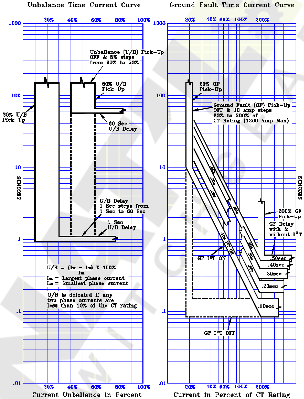
Figure 4 Unbalance TCC & Ground Fault TCC
