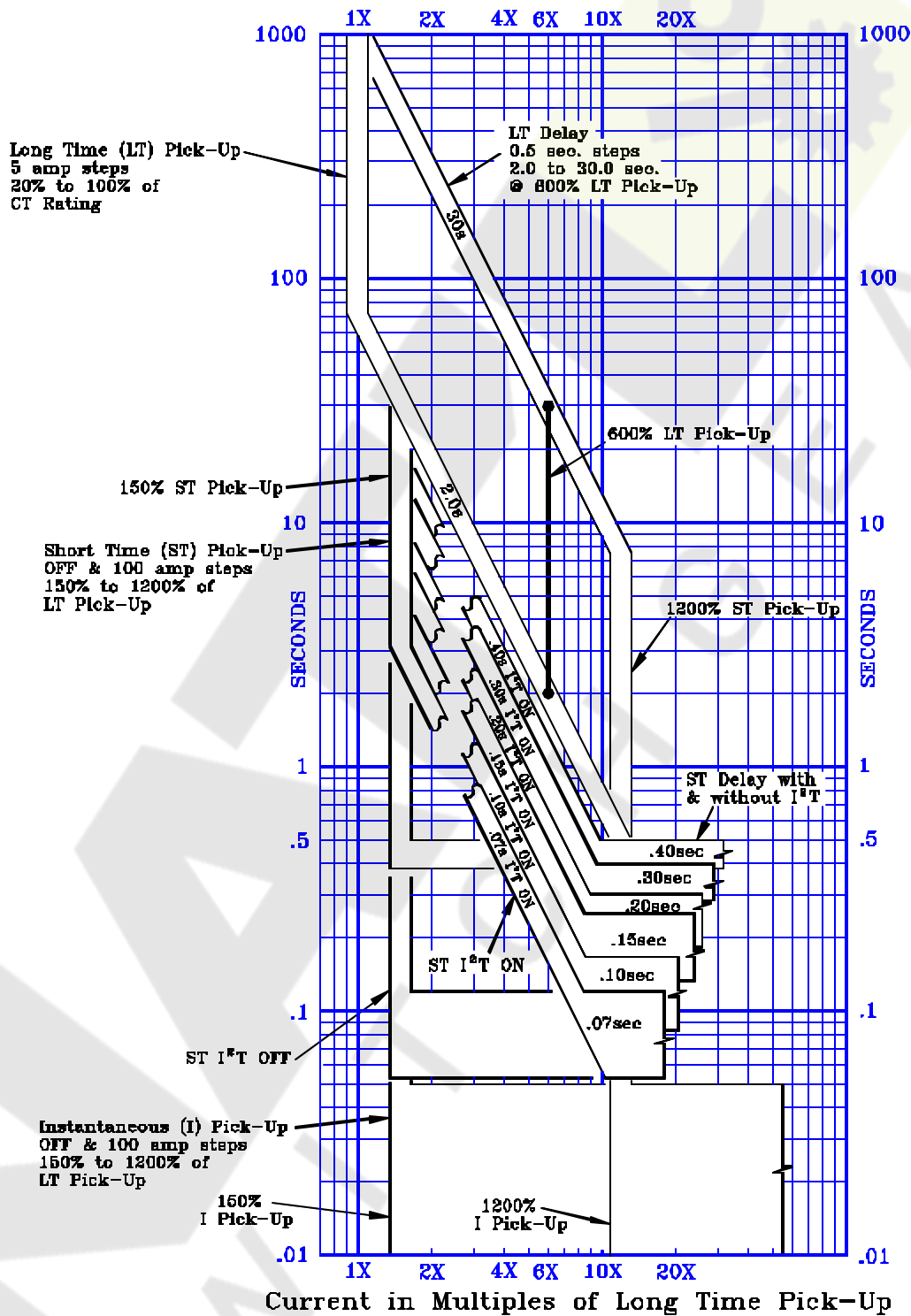
Figure 5 Overload TCC
